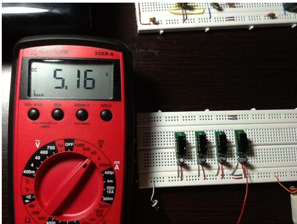
Photo 3. measuring the output voltage of one of the distance sensors without obstruction
