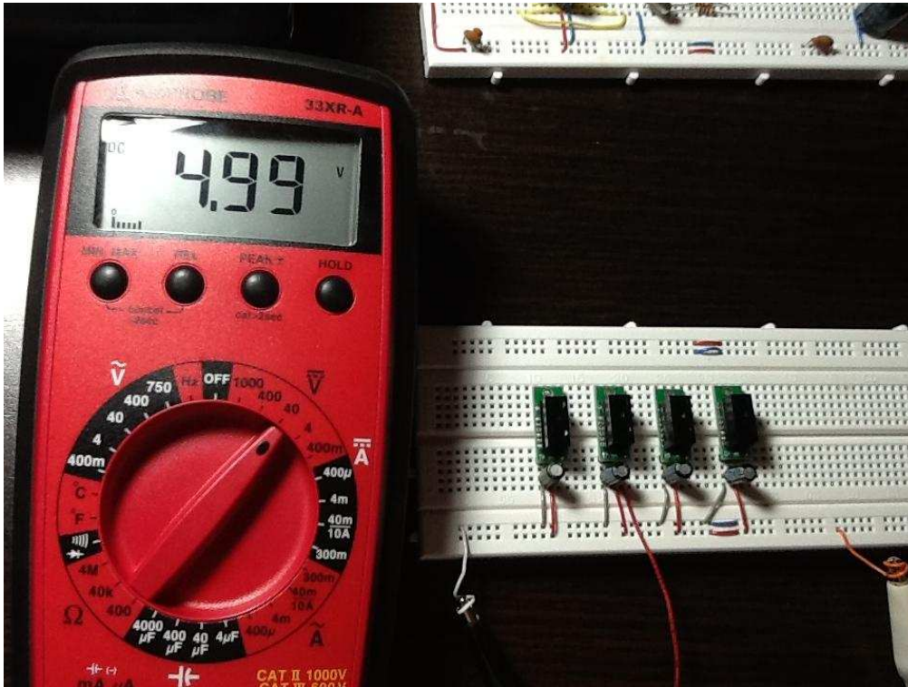
Photo 4. measuring the output voltage of another sharp distance sensors without obstruction
